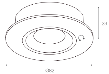
GU10 W 1XGU10 Max. 50W
